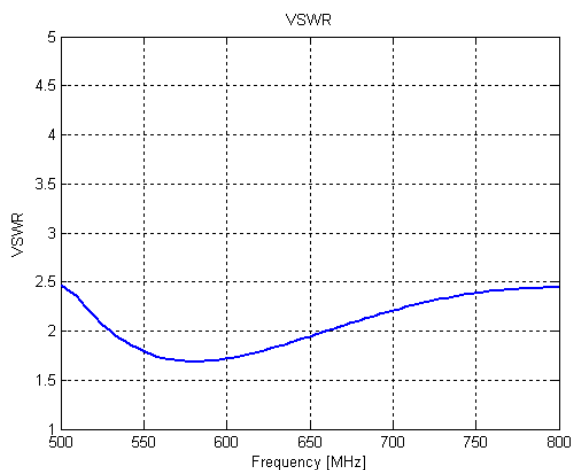
Typical VSWR
