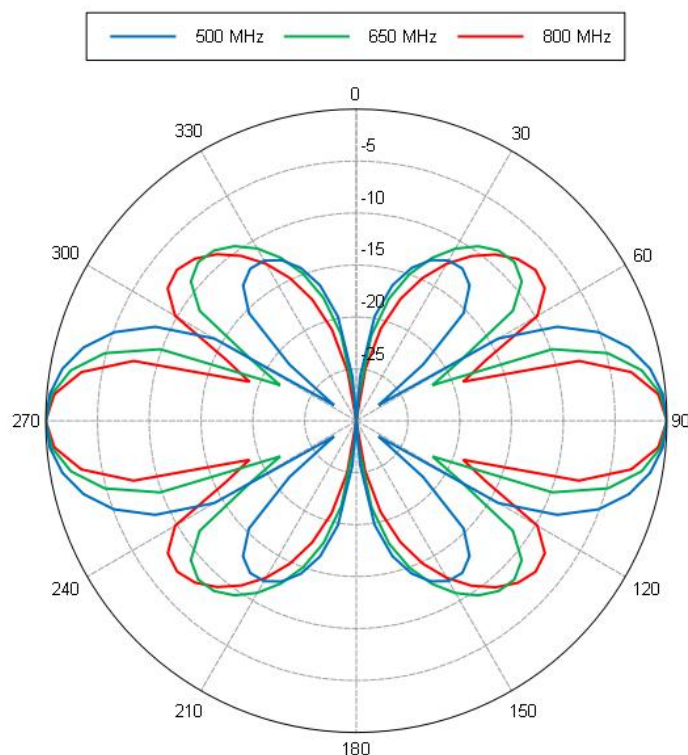
Elevation Patterns
