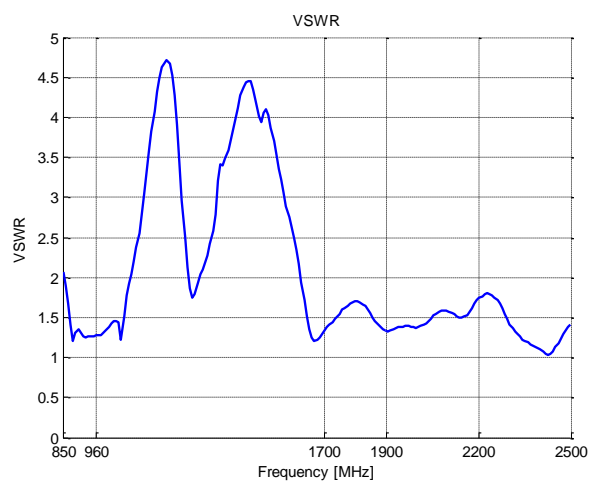
Typical VSWR
