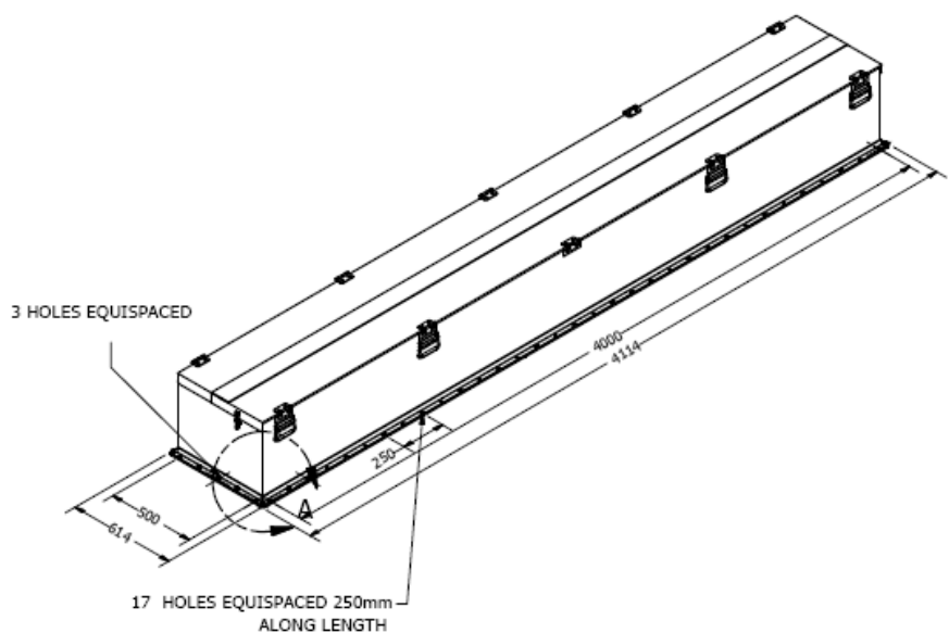
Antenna assembly enclosure ICD
